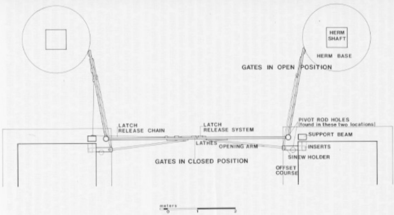
76 Plan showing gates in open and closed positions, Lepcis Magna
